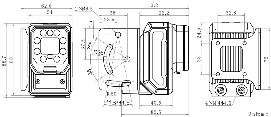
Installation Bracket:
