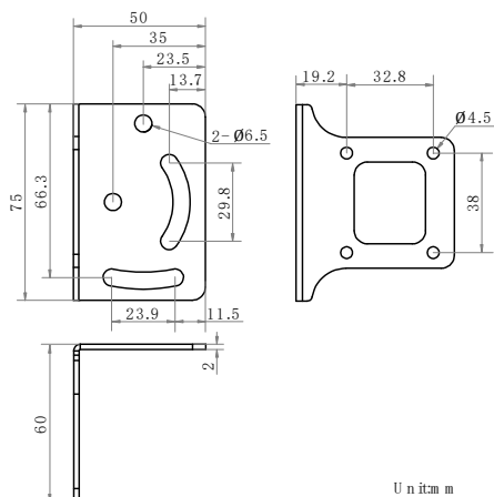
Installation Bracket:
